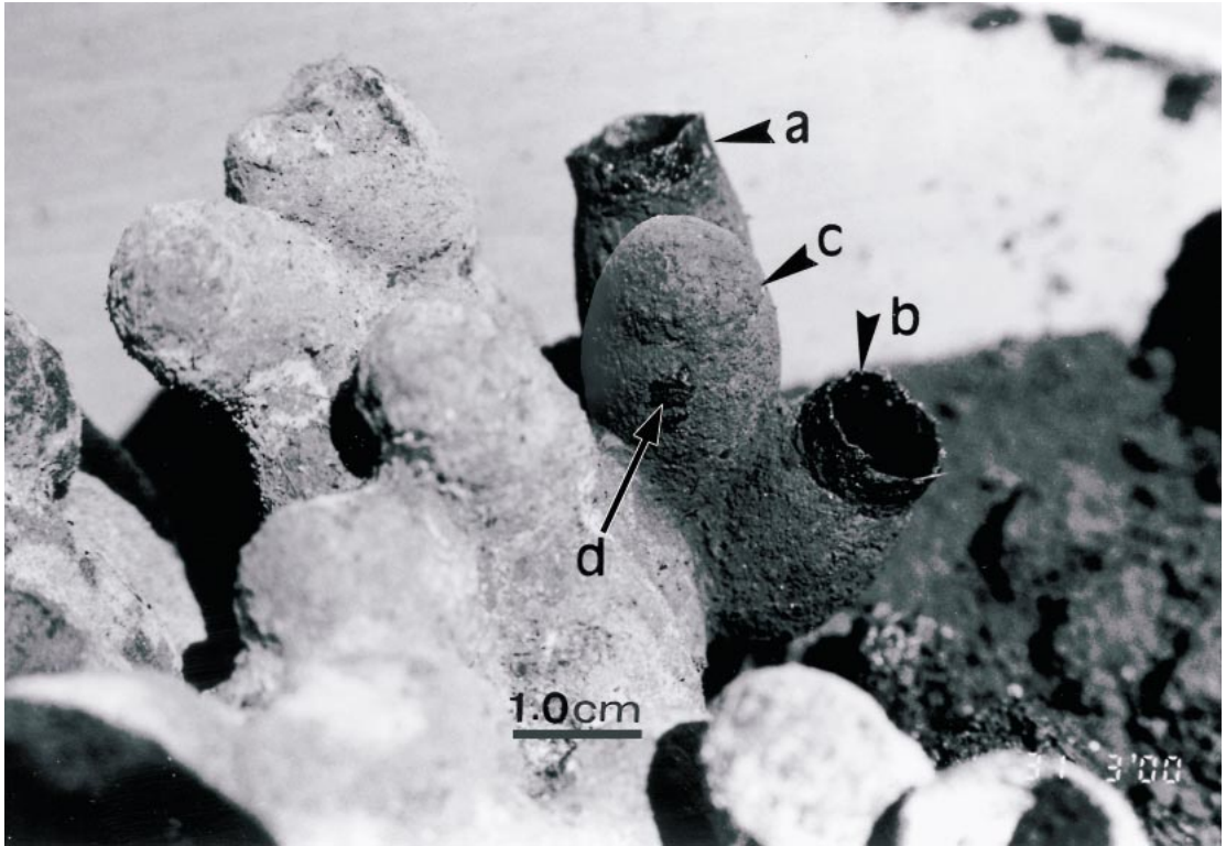
Fig. 1. Cells of Eulaema nigrata being provisioned (a and b) and parasitized (c) by Exaerete smaragdina ; the arrow (d) indicates the plugged scar made by Exaerete smaragdina . The new cells (a, b, and c) were attached to one cell of the older cell cluster built during the first re-use process of N-6.
